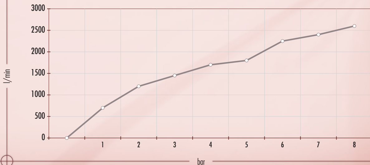
GRAFICO CONSUMO ARIA RUBINETTI UNIVERSALI A RULLI - DUAL PIN TYPE COUPLERS AIR CONSUMPTION GRAPH GRAPHIQUE CONSOMMATION D'AIR RACCORDS RAPIDES A AIGUILLE
